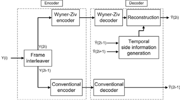
Figure 1. Non-scalable DVC scheme (GOP=2).
