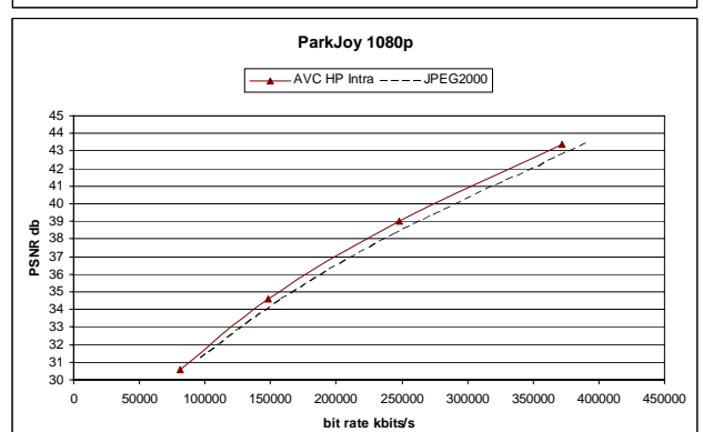
Fig.5. Rate-distortion for ParkJoy.
