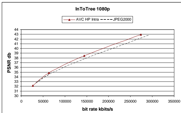
Fig.3. Rate-distortion for InToTree.
