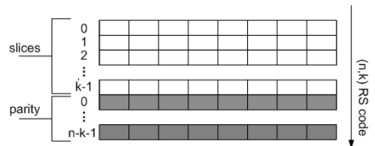
Fig. 4. Reed-Solomon code application scheme.
